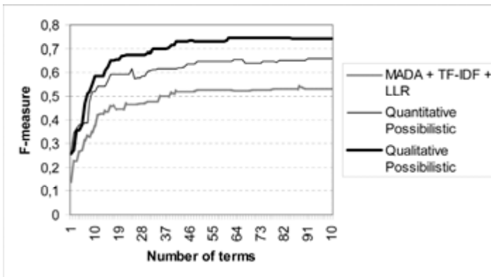
Figure 8. The curves of F-measure for the domain of purification (All terms)
