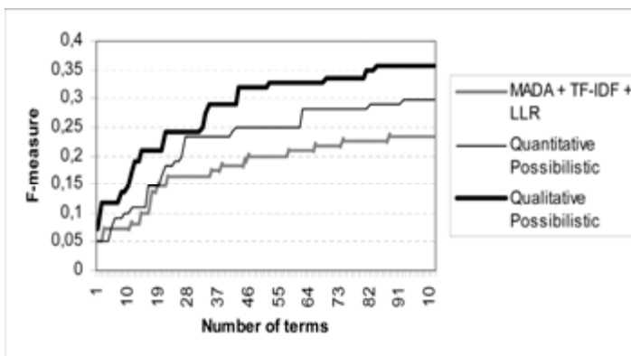
Figure 9. The curves of F-measure for the domain of purification (MWTs).
