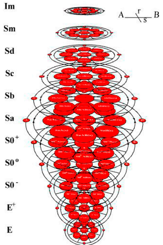
Figure 1. The de Vaucouleurs system. This table is an attempt to produce a more versatile form of simpler classification tables for galaxies (specifically the Hubble “Tuning Fork” diagram), but it is not a true 3D graph. The galaxy types (Im through E) do not represent, at present, known quantifiable parameters. Neither do the other two indexes (family and variety). This system is, nevertheless, an illustration of the greater versatility of 3D classification tables. (This table is a simulation; apparently no fully developed table actually exists.) Note the similarity to the Stowe table.
