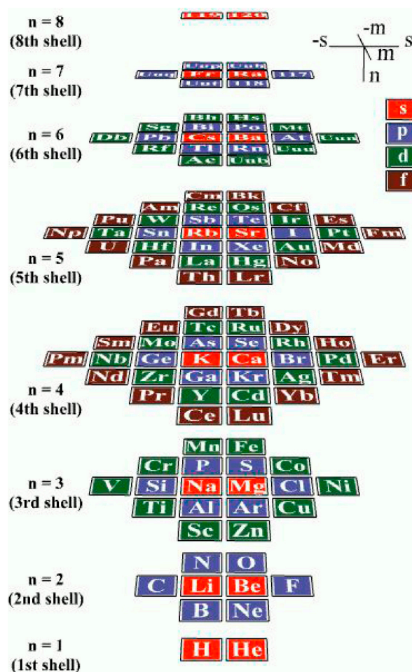
Figure 2. The Stowe Periodic Table. The parameters are the three quantum numbers, n (shell), s (spin) and m (orientation), the fundamental determinants of atomic structure and properties. Notice the perfect symmetry. All classes, groups and "blocks" fall into perfect rings, columns or levels. The 3D, interactive version ( www.projectcosmology.net ) provides simple, on-screen controls for manipulation and isolation of rings, columns and levels. Each individual symbol is a link to some 100 categories of data. In time, each symbol will also provide access to energy level diagrams, 3D, interactive orbital schematics, and lists of formulae for quantum mechanics. (Due to budgetary constraints, only hydrogen is fully developed at this time.)
